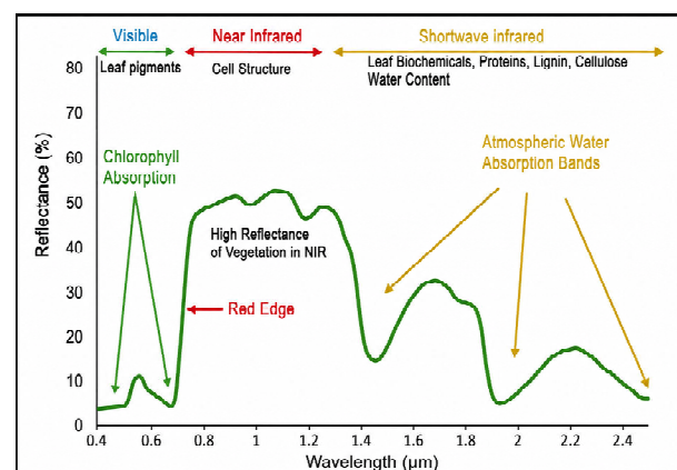
Fig.1: Schematic diagram of spectral signature of vegetation (Source: Roman and Ursu, 2016)
