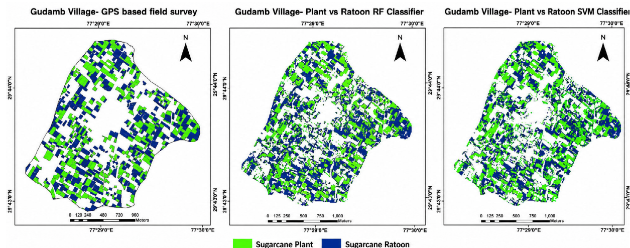
Fig. 3: Comparison of Plant and Ratoon Crop Classification with GPS Survey Data in Gudamb Village, KSCM Catchment (Source: Nihar et al. , 2022)
