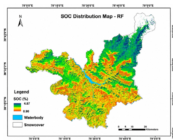
Fig. 5: Spatio-temporal map of SOC predicted by RF model in the study area (Source: Kalambukattu et al. , 2025)
