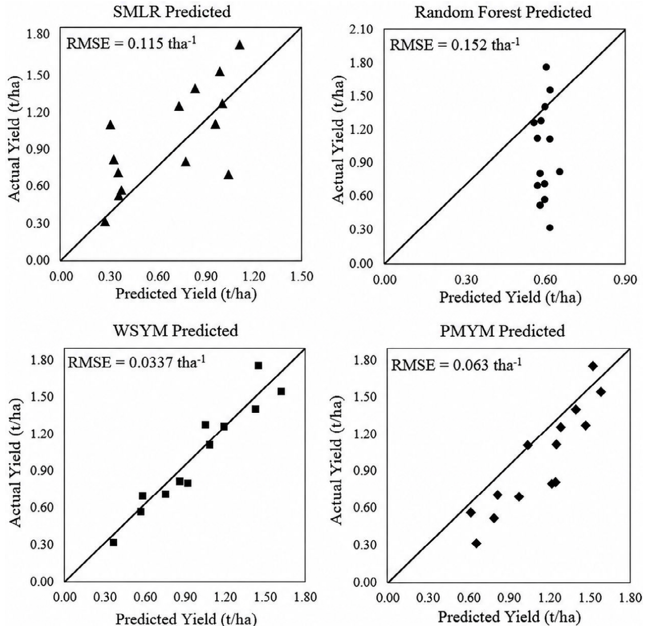
Fig. 4: Performance Comparison of Various Models for Field Pea Yield Prediction (Source: Danodia et al. , 2025)
