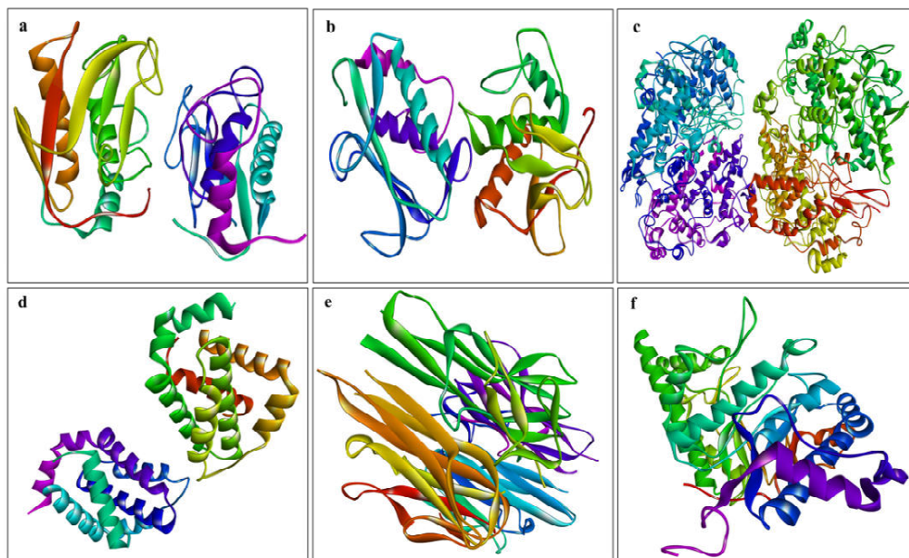
Fig. 1: 3D structures of target protein molecules. (a): Metalloproteinase-1 (PDB ID: 1CGL), (b): Matrix Metalloproteinase-9 (PDB ID: 1GKC), (c): Cyclooxygenase-2 (PDB ID: 4COX), (d): B-cell lymphoma 2 (PDB ID: 4MAN), (e): Tumor Necrosis Factor-alpha (PDB ID: 2AZ5), (f): Hyaluronidase-1 (PDB ID: 2PE4)
