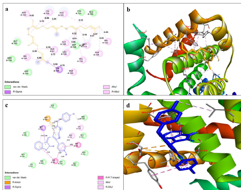
Fig. 5: Two-dimensional (2D) molecular interaction maps and three-dimensional (3D) binding poses of squalene and the reference inhibitor disparib within the binding pocket of B-cell lymphoma-2 (Bcl-2; PDB ID: 4MAN). (a) and (b) represent the 2D interaction map and 3D binding pose of squalene, while (c) and (d) represent those of disparib. The interaction maps identify the amino acid residues participating in ligand binding and corresponding interactions, whereas the 3D structures illustrate the spatial orientation of the ligands within the binding cavity. The Fig. facilitates comparison of the binding modes and interaction profiles of squalene and disparib with Bcl-2
