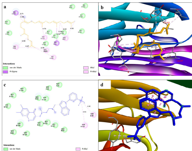
Fig. 6: Two-dimensional (2D) molecular interaction maps and three-dimensional (3D) binding poses of squalene and the reference inhibitor SPD304 within the binding pocket of tumour necrosis factor-alpha (TNF- \alpha ; PDB ID: 2AZ5). (a) and (b) represent the 2D interaction map and 3D binding pose of squalene, while (c) and (d) represent those of SPD304. The interaction maps identify the amino acid residues participating in ligand binding and corresponding interactions, whereas the 3D structures illustrate the spatial orientation of the ligands within the binding cavity. The Fig. facilitates comparison of the binding modes and interaction profiles of squalene and SPD304 with TNF- \alpha
